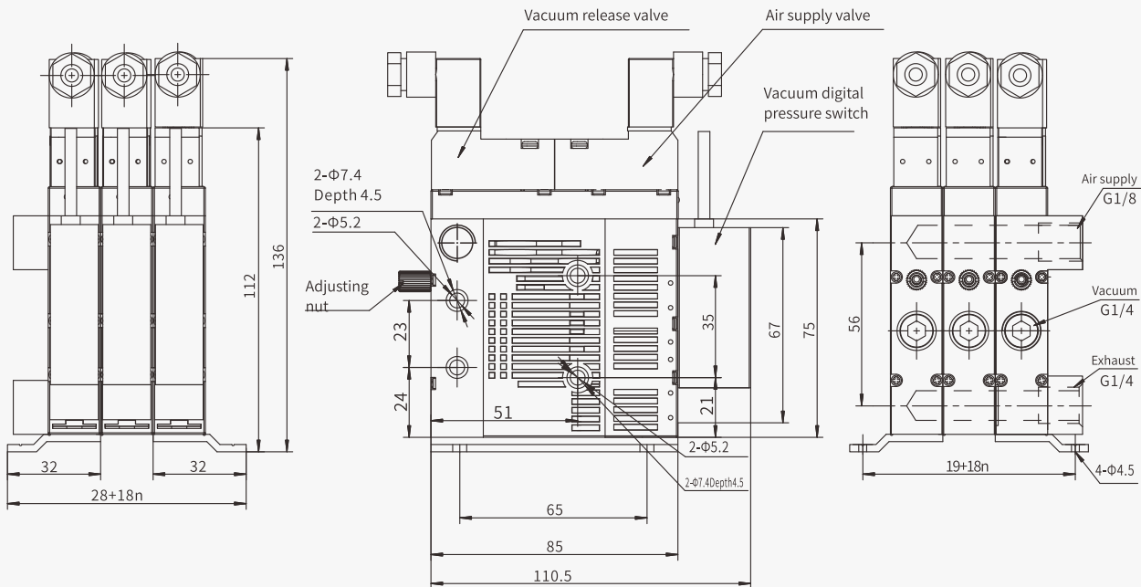
Concentrated air supply+Concentrated exhaust
