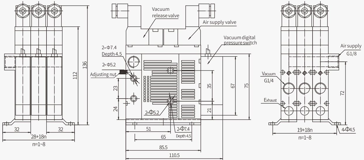
Concentrated air supply + Individual exhaust
