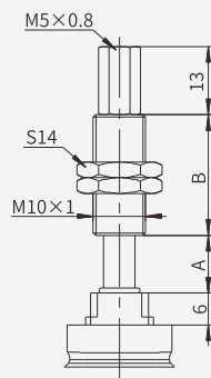
Suction cup 4×20 5×20 6×20 8×20
