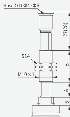
Suction cup 4×20 5×20 6×20 8×20
