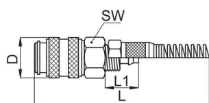
Coupling with bulkhead hose adapter
