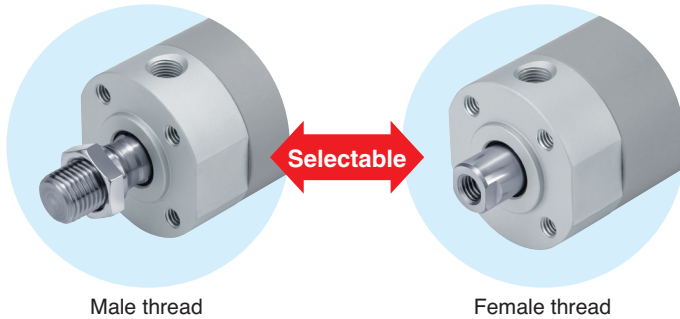
Male thread
