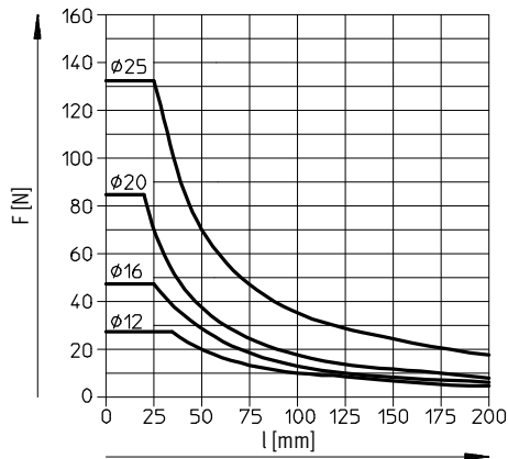
DFM-12 ... 25-KF Stroke 30 mm
