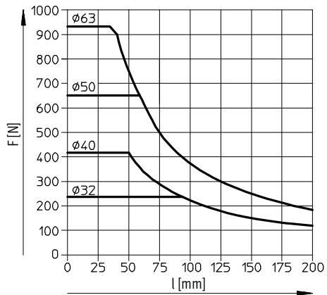
DFM-32 ... 63-GF Stroke 50 mm
