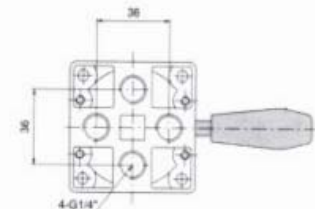
Base mounting style
