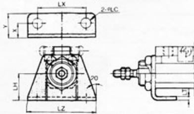
Flange Style
