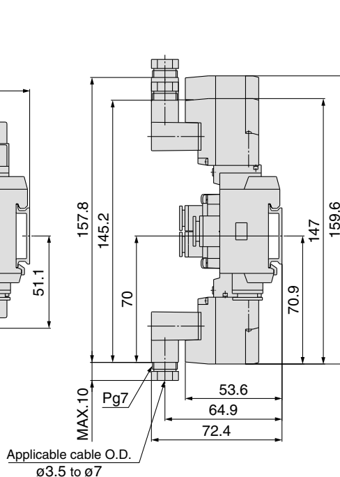
M plug connector (M)
